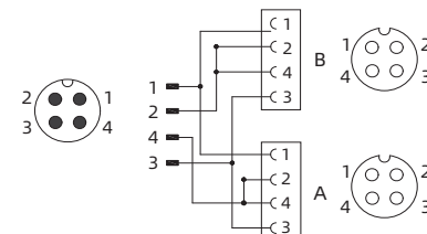
M12Y3型连接器电路图
