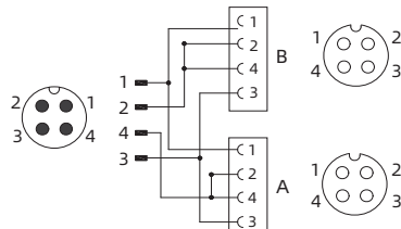
M12Y3型连接器电路图
