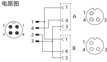
M12Y2型连接器电路图
